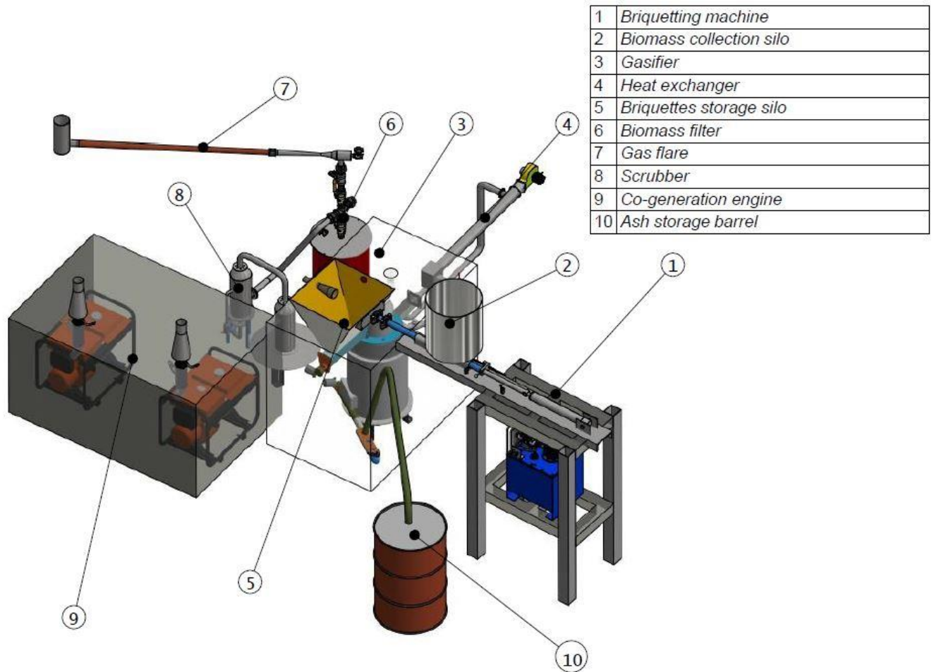
3D illustration of the gasification system
